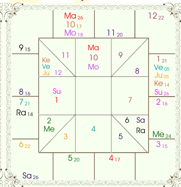
Cusp Chart
