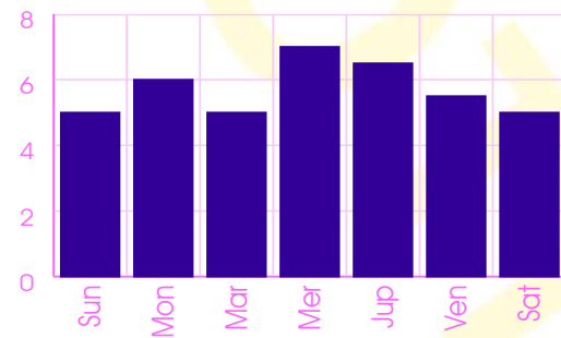
Minimum Shadbala
