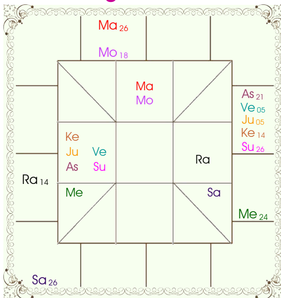
Lagna Chart
