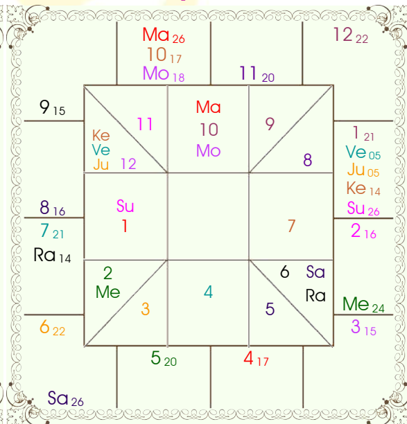
Cusp Chart
