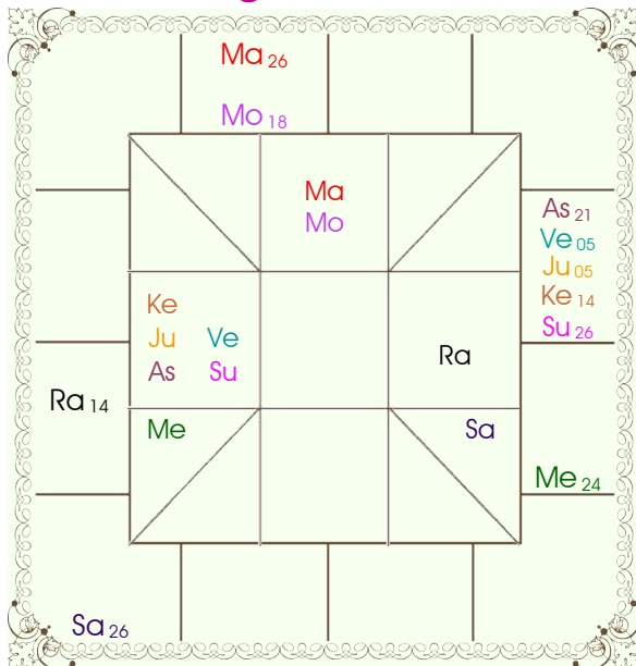
Lagna Chart
